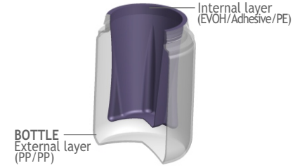
AirFree® multilayer bottle Bag-in-bottle airless system
